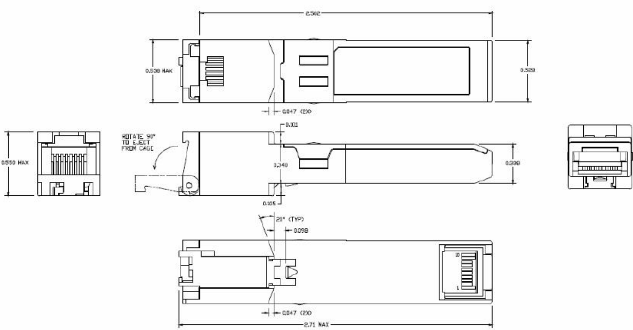
Figure 2. mechanical dimensions
