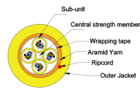
Structure Diagram
