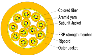
Structure Diagram
