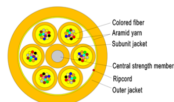
Structure Diagram
