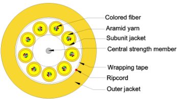
Structure Diagram
