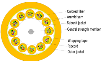
Structure Diagram
