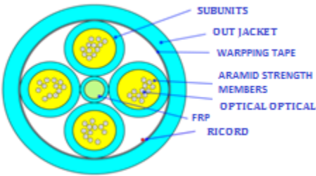
Structure Diagram
