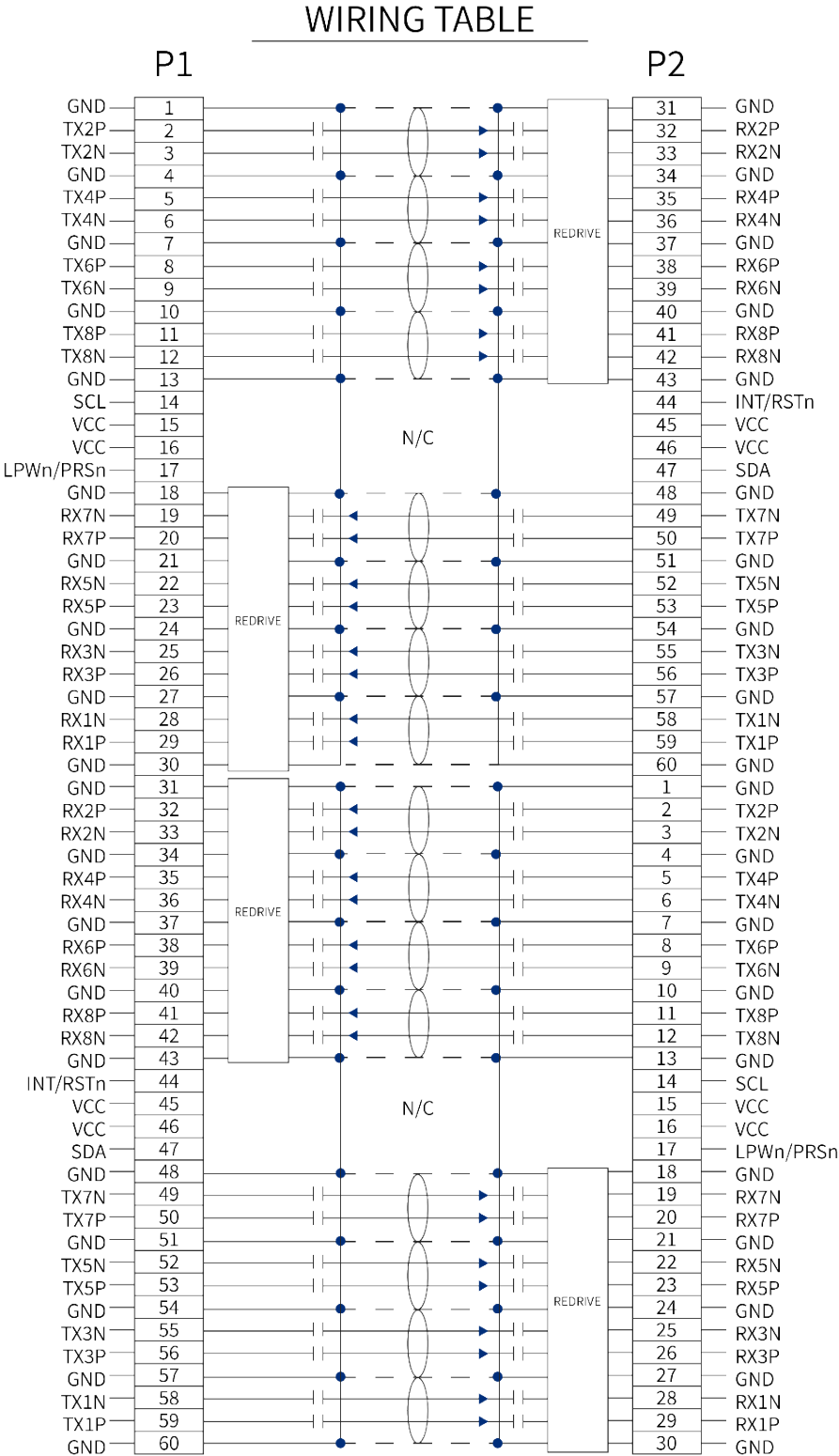
Figure 2 OSFP 400G Active Redriver Cable Assembly Wiring
