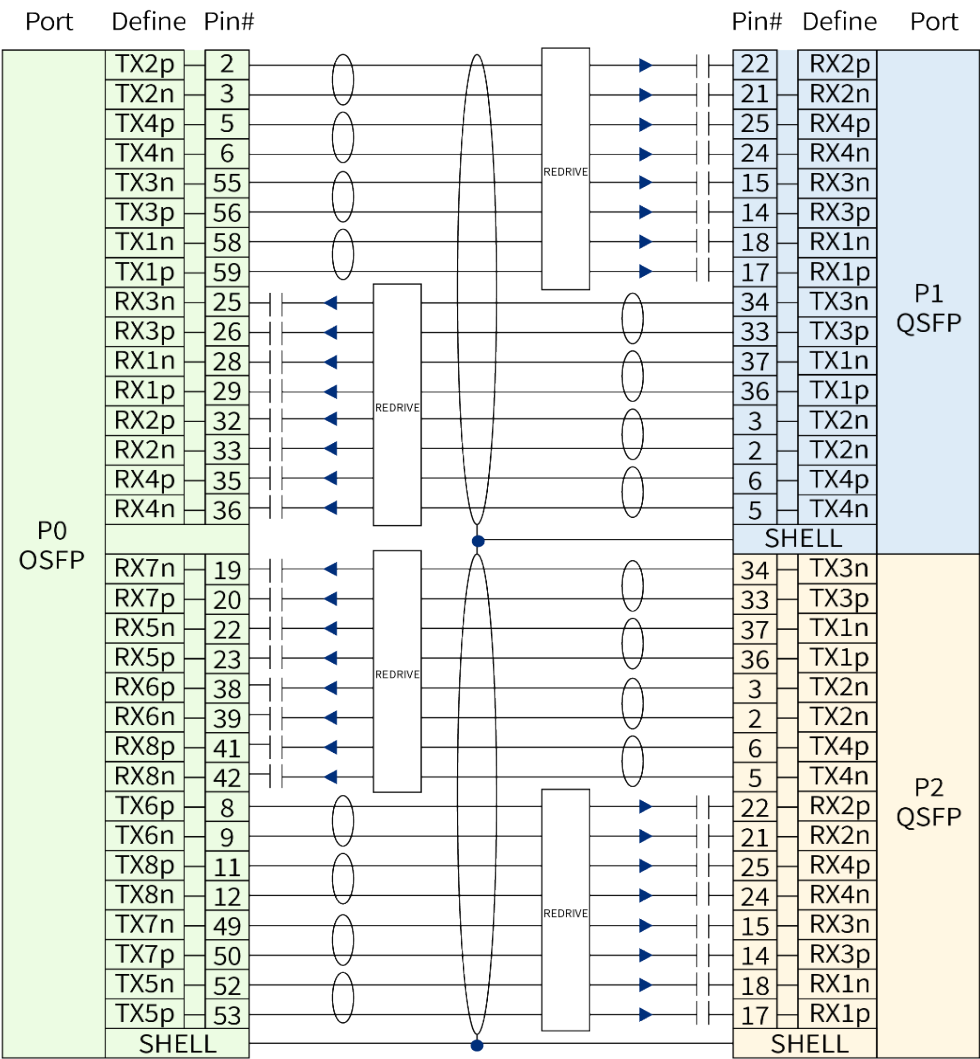
Figure 3 OSFP 400G to 2*QSFP56 Active Redriver cable Wiring
