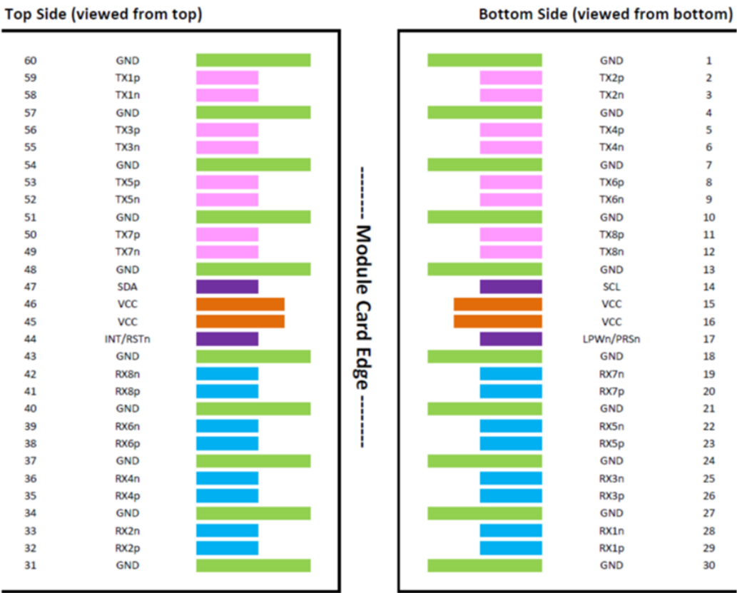
Figure 1 OSFP/OSFP-RHS Module Contact Assignment
