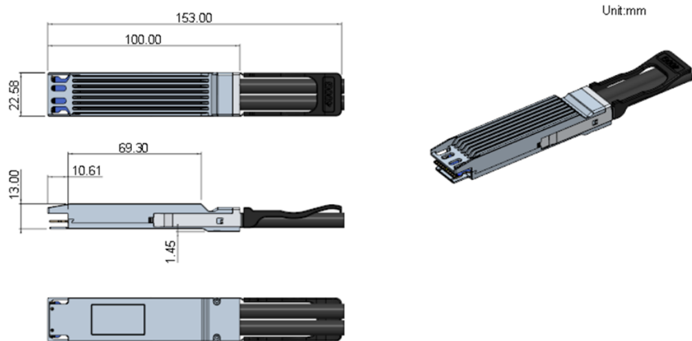
Figure 5 OSFP Form Factor
