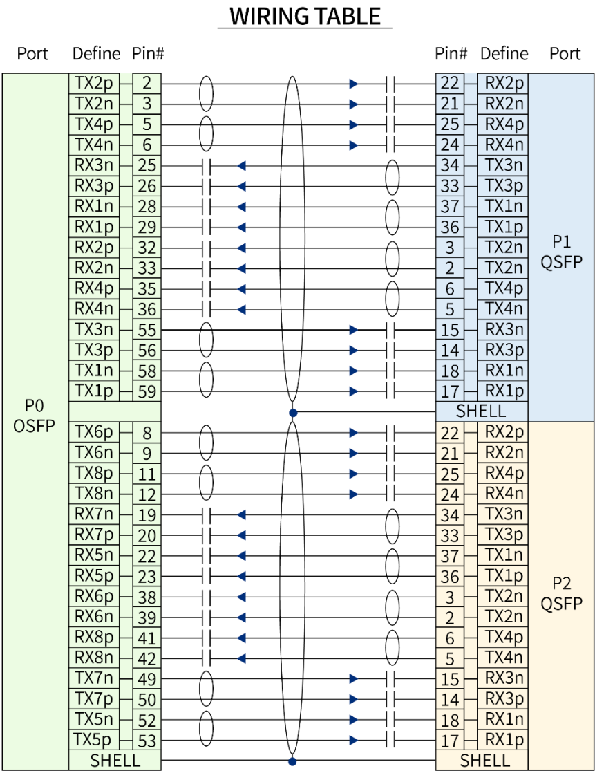
Figure 3 OSFP 400G to 2*QSFP56 Direct Attached cable Wiring
