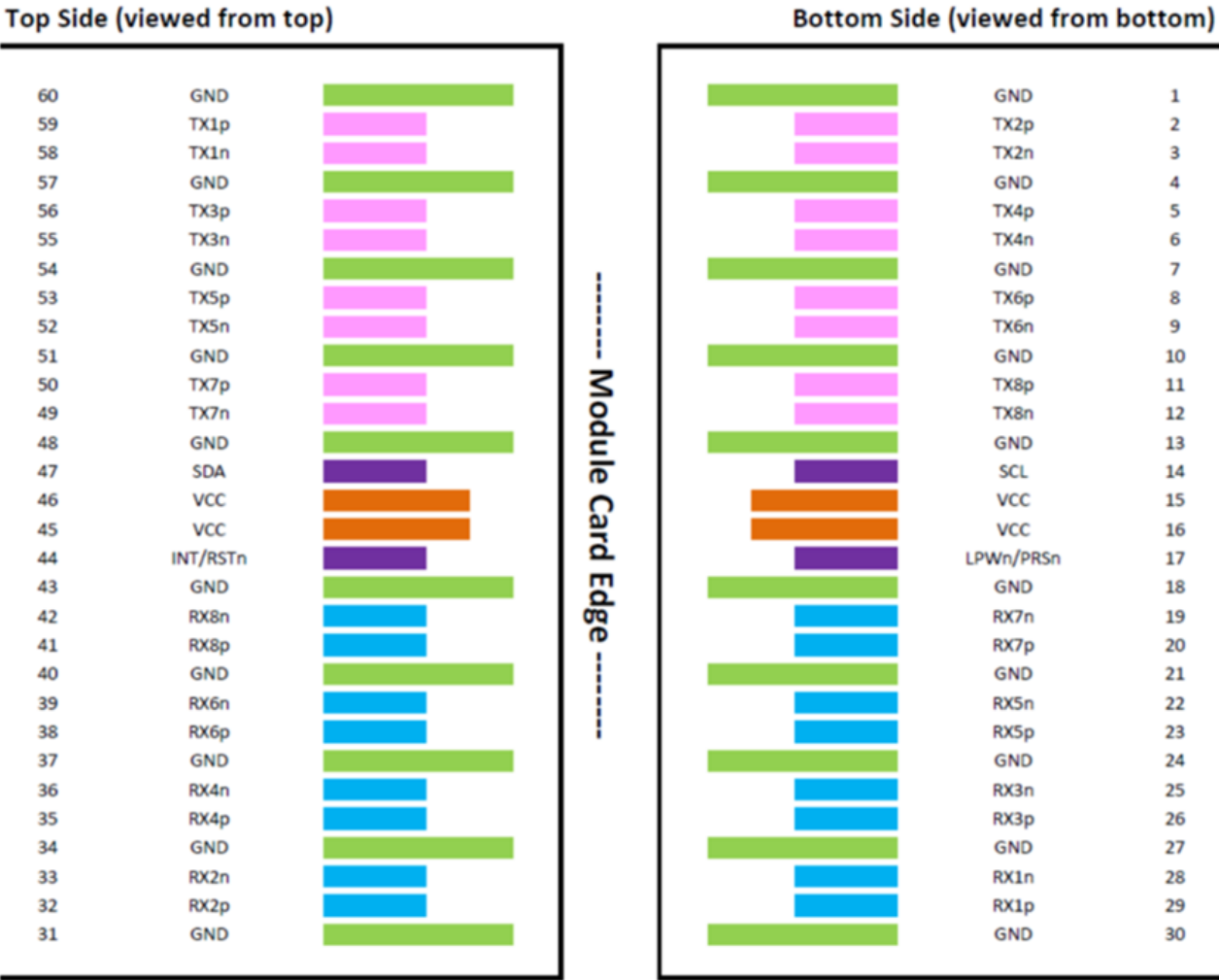
Figure 1 OSFP Module Contact Assignment
