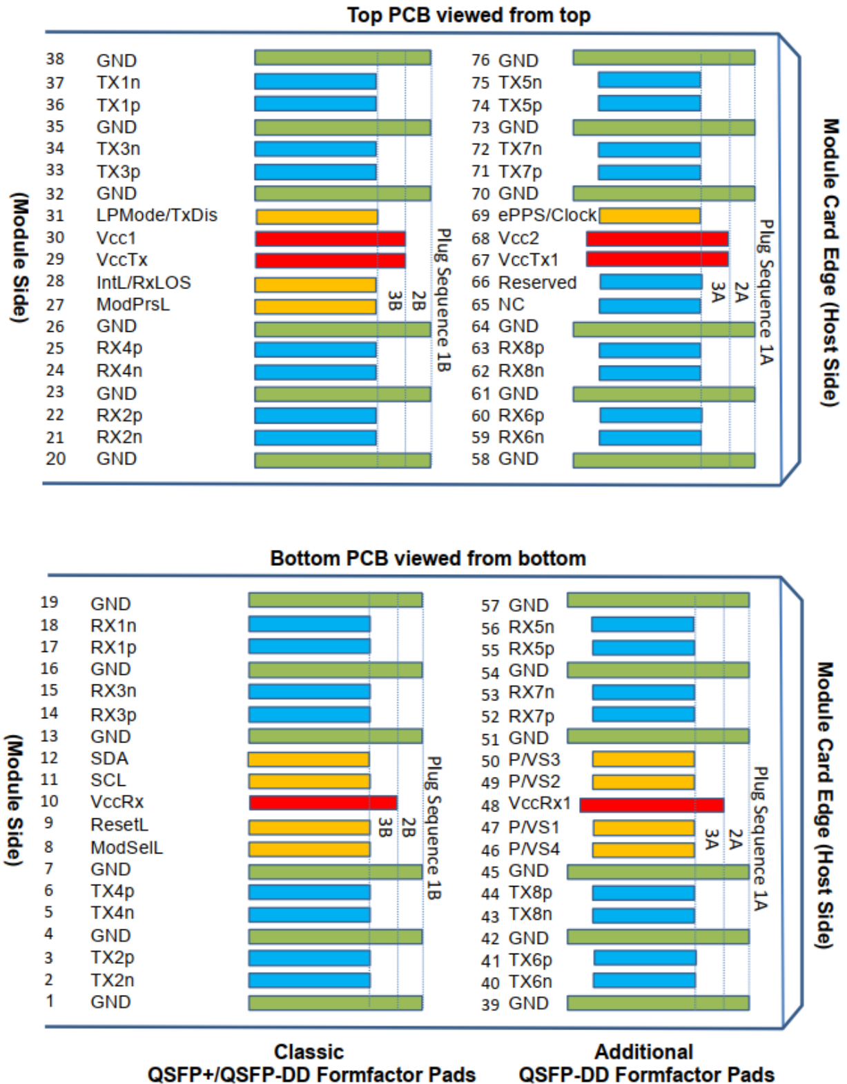
Figure 2 QSFP-DD Module Contact Assignment
