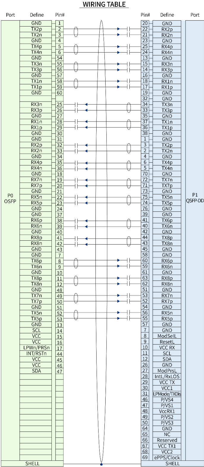
Figure 3 OSFP/OSFP-RHS to QSFP-DD (400G) Direct Attached cable Wiring
