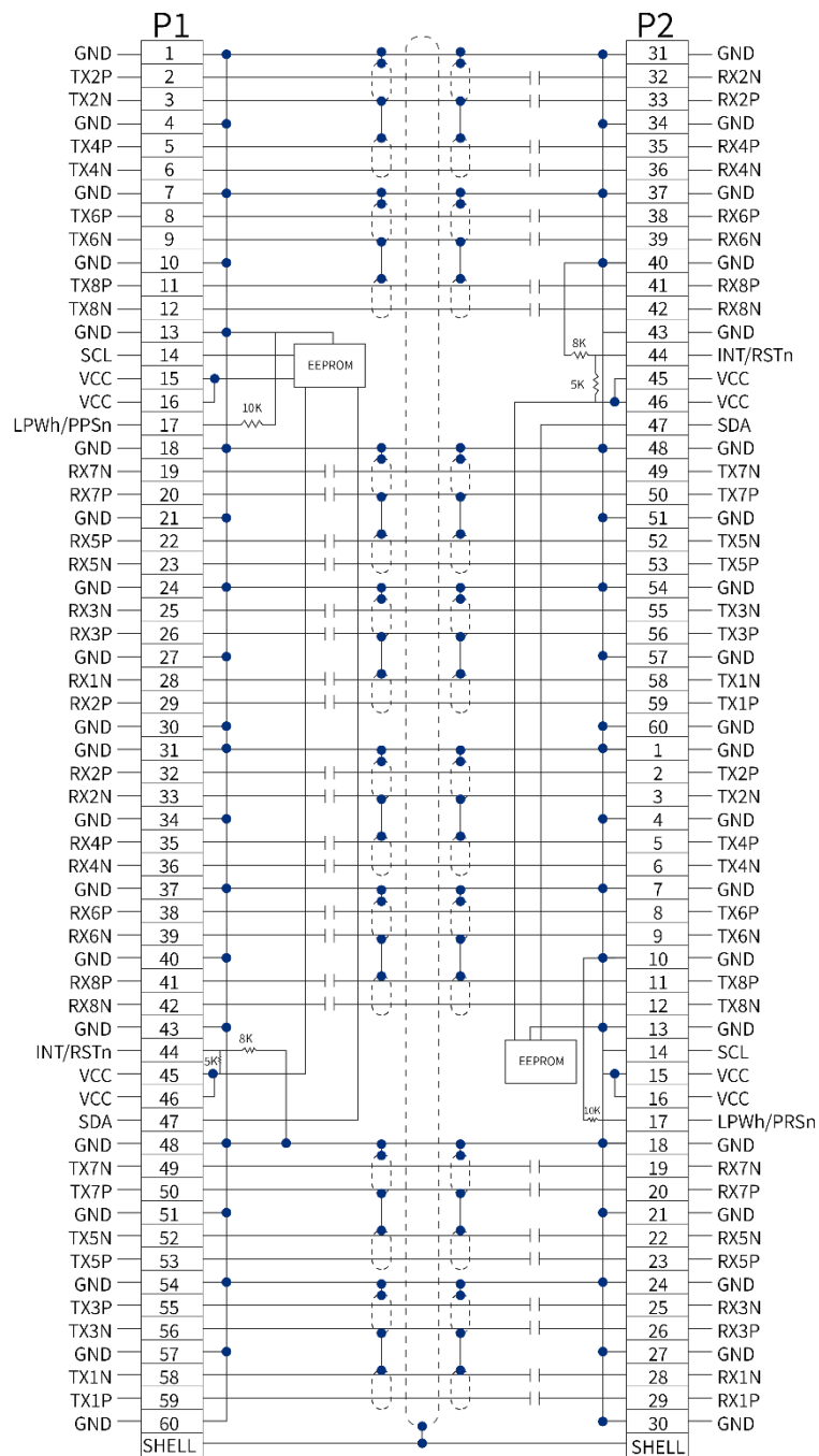
Figure 2 OSFP 800G Direct Attached Cable Assembly Wiring
