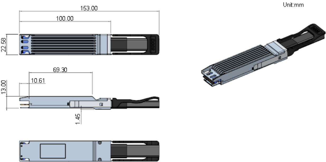
Figure 4 OSFP800 Form Factor
