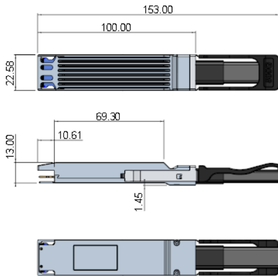
Figure 4 OSFP 800 Form Factor (P0 End)
