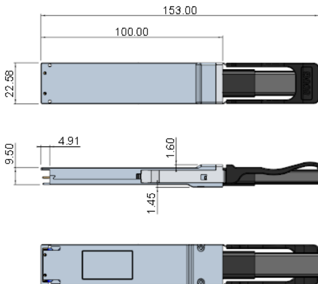
Figure 5 OSFP-RHS Type Form Factor (P1&amp;P2 End)
