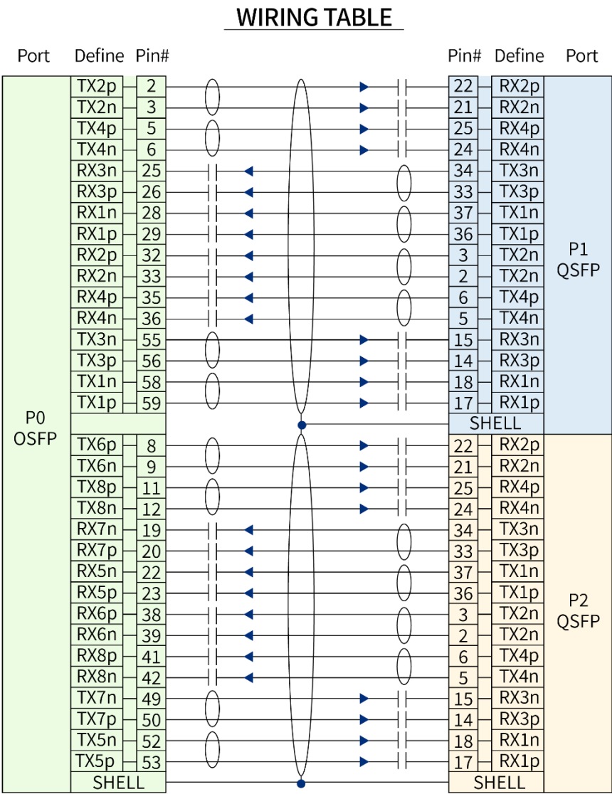
Figure 3 OSFP 800G to 2*QSFP112 (4*100G) Direct Attached Cable Assembly Wiring
