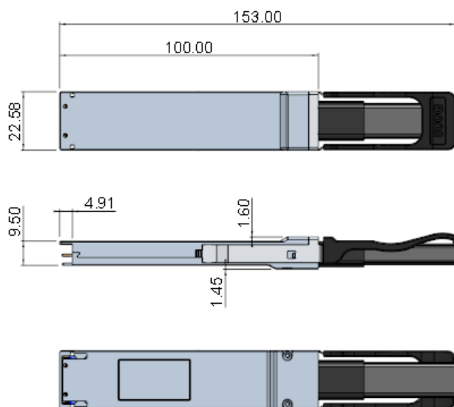
Figure 5 OSFP-RHS Type Form Factor (P1~P4 End)
