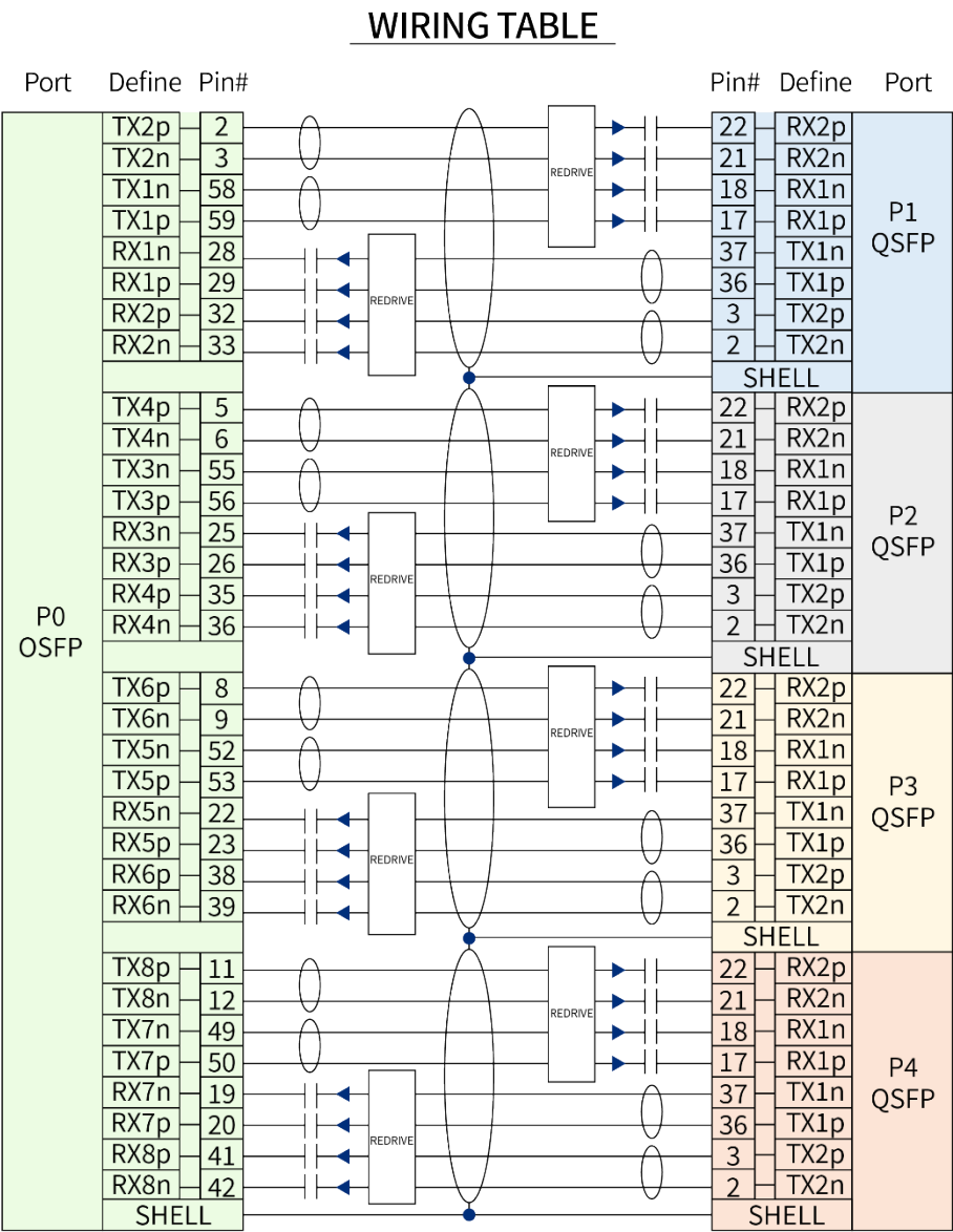
Figure 3 OSFP 800G to 4*QSFP112 (2*100G) Active Redriver Cable Assembly Wiring
