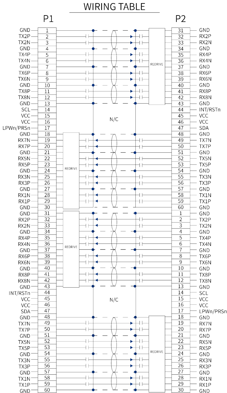
Figure 2 OSFP-RHS 400G Active Redriver Cable Assembly Wiring
