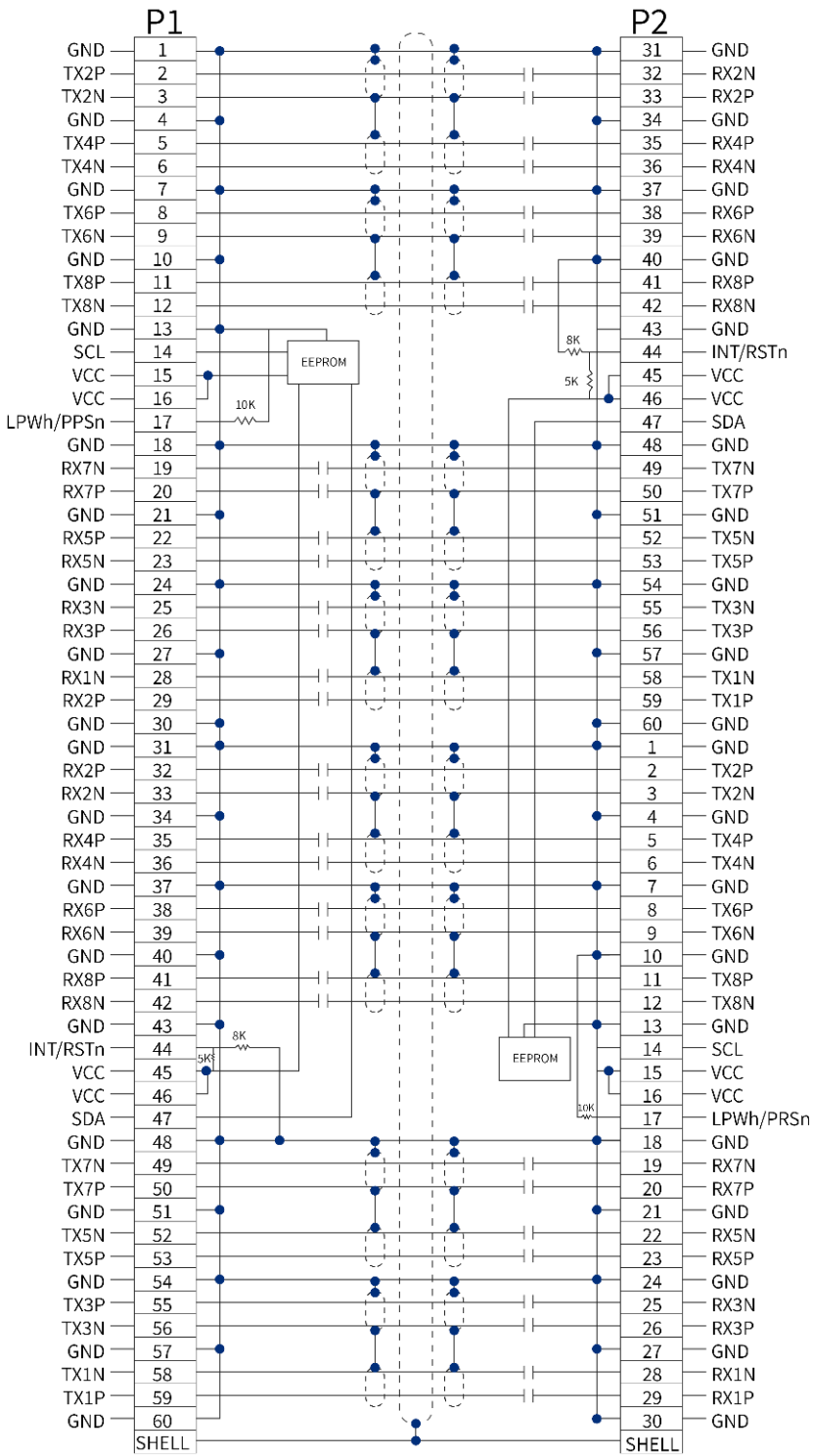
Figure 2 OSFP-RHS 800G Direct Attached Cable Assembly Wiring
