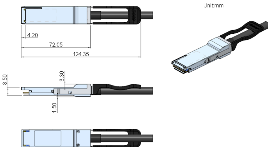
Figure 6 QSFP112 Type Form Factor
