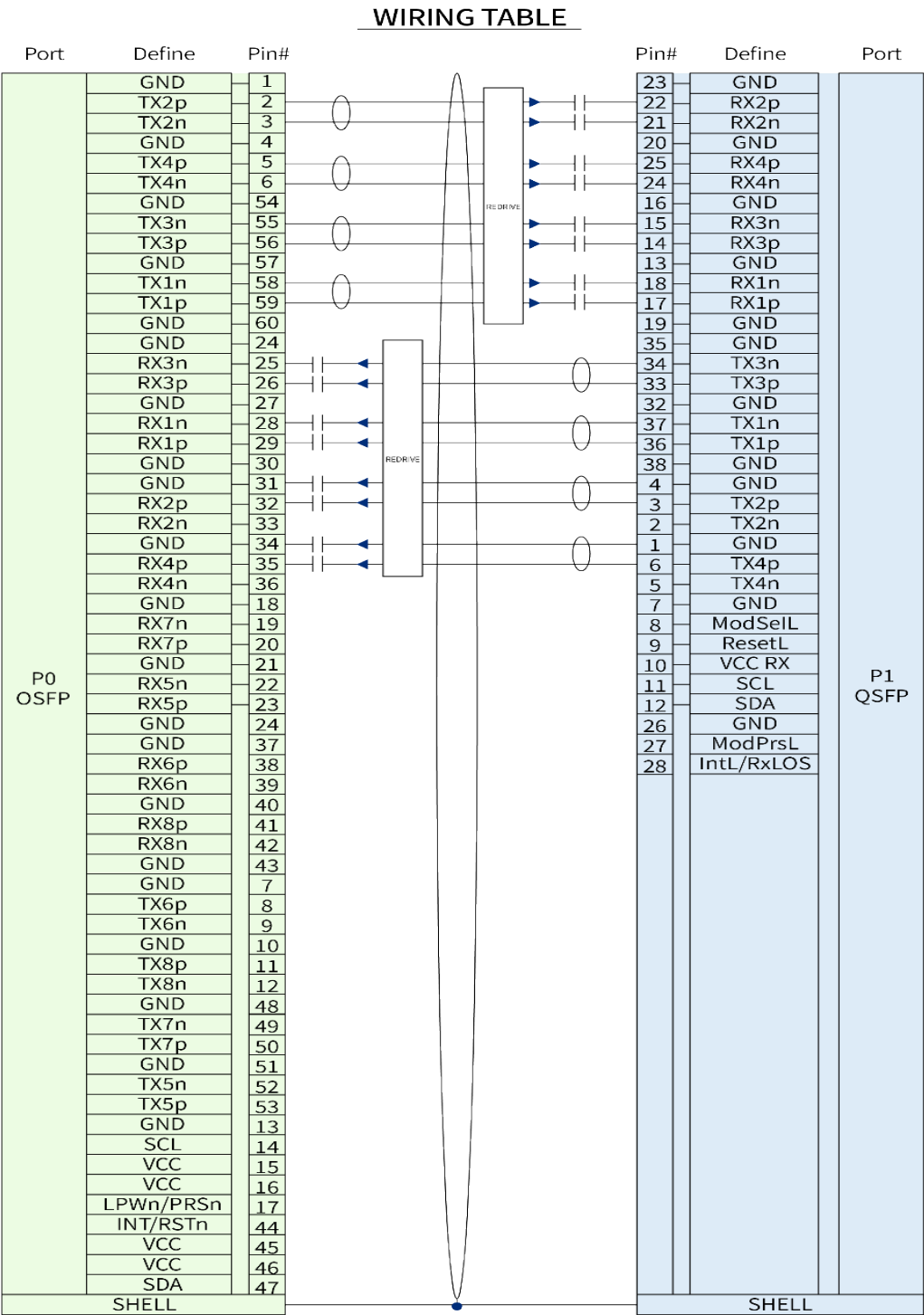
Figure 3 OSFP-RHS800 to 1*QSFP112 Active Redriver Cable Assembly Wiring
