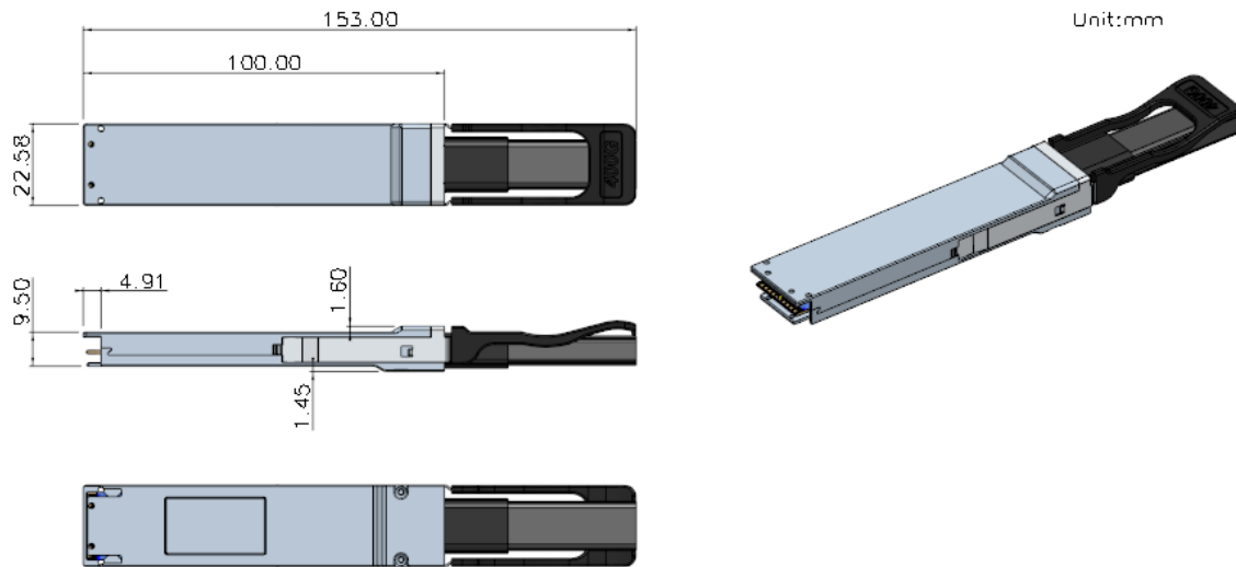
Figure 5 OSFP-RHS 800 Form Factor
