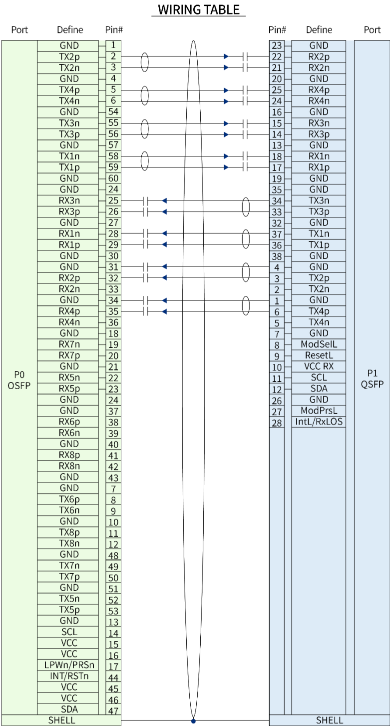
Figure 3 OSFP-RHS800G to 1*QSFP112 Direct Attached Cable Assembly Wiring
