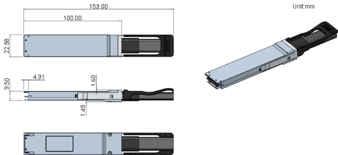
Figure 5 OSFP-RHS 800 Form Factor (P0 End)
