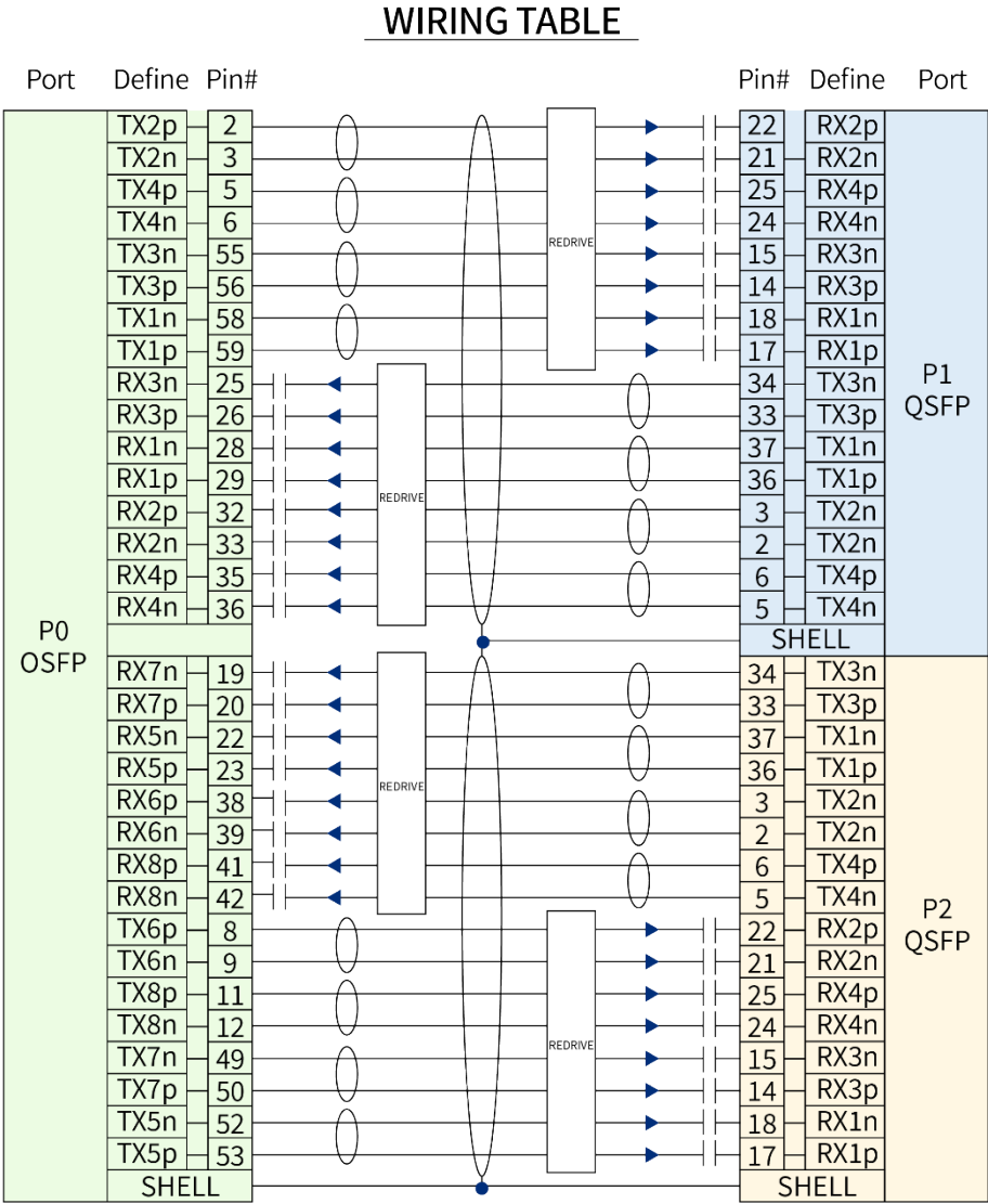
Figure 3 OSFP-RHS 800G to 2*QSFP112 (4*100G) Active Redriver Assembly Wiring
