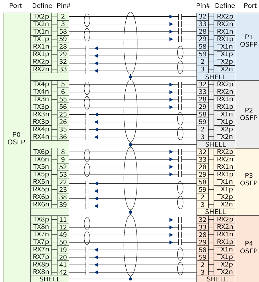
Figure 2 OSFP 800G to 4*OSFP-RHS (2*100G) Direct Attached Cable Assembly Wiring
