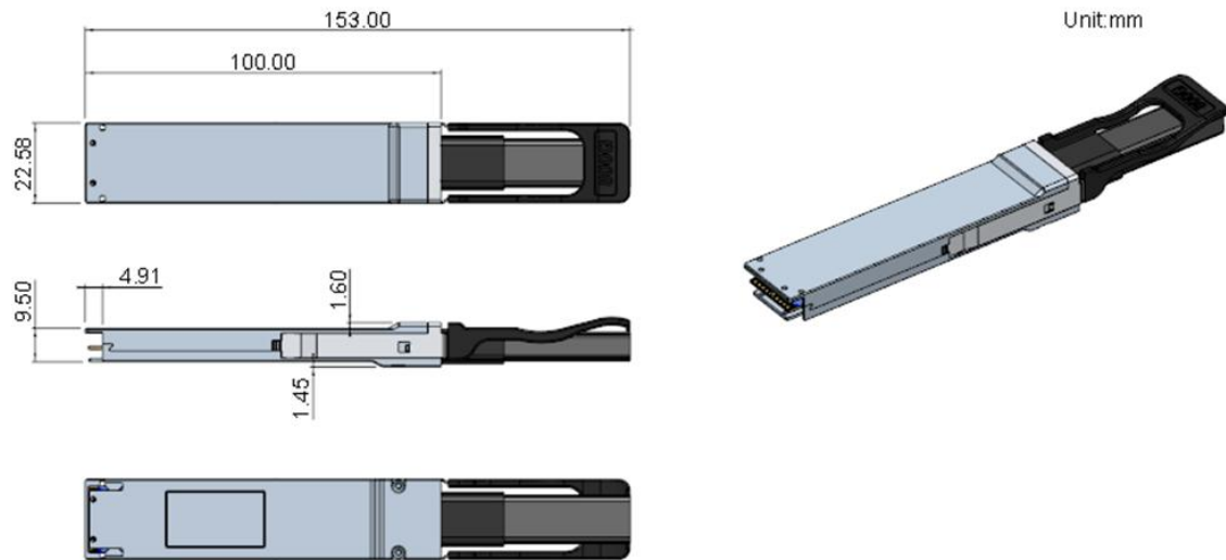
Figure 4 OSFP-RHS 800 Form Factor (P0~P5 End)
