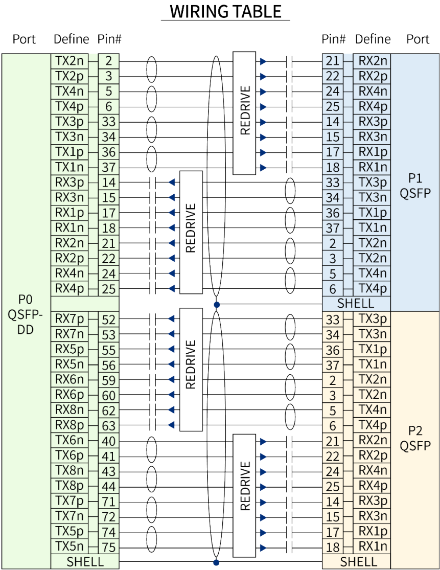
Figure 3 QSFP-DD 400G to 2*QSFP56 Active Redriver cable Wiring
