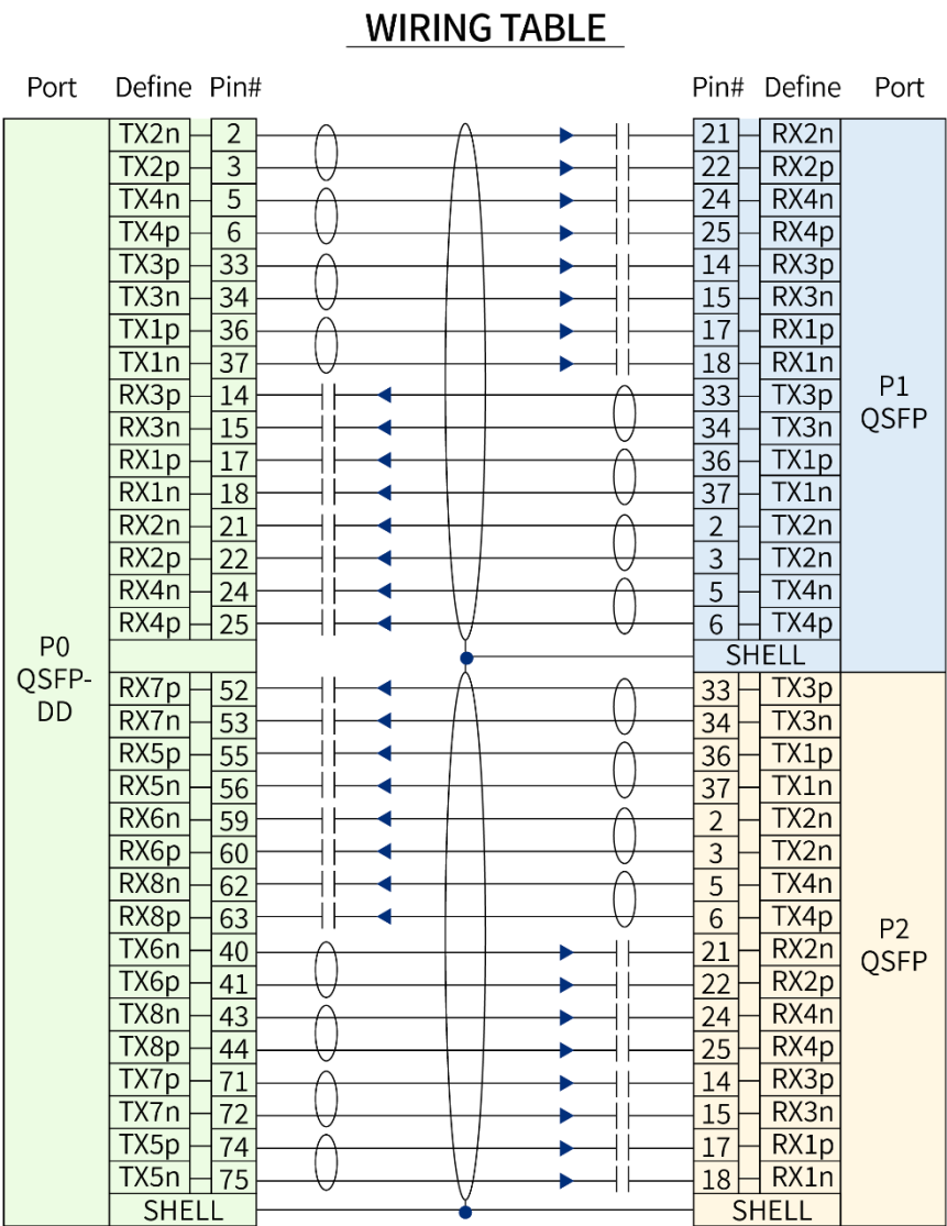
Figure 3 QSFP-DD 400G to 2*QSFP56 Direct Attached cable Wiring
