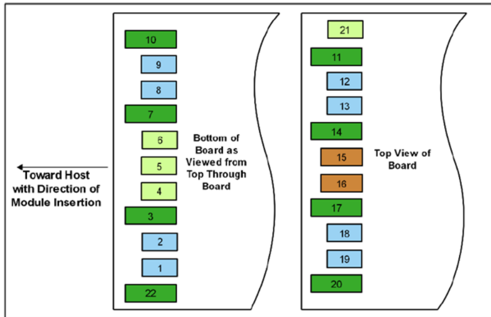
Figure 2 DSFP28(56) Module Contact Assignment
