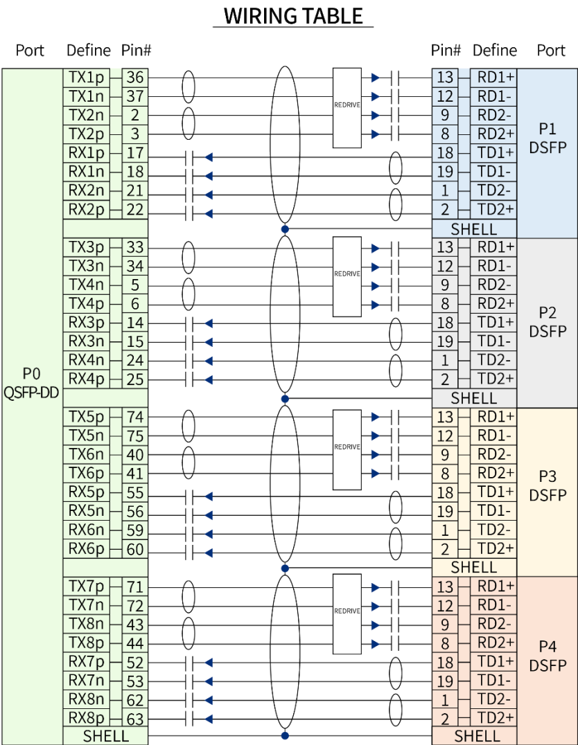
Figure 3 QSFP-DD 400G to 4*DSFP56 Active Redriver cable Wiring
