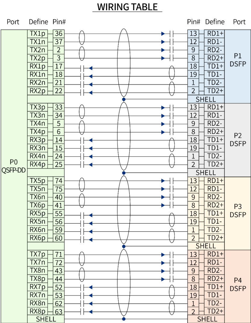
Figure 3 QSFP-DD 400G to 4*DSFP56 Direct Attached cable Wiring
