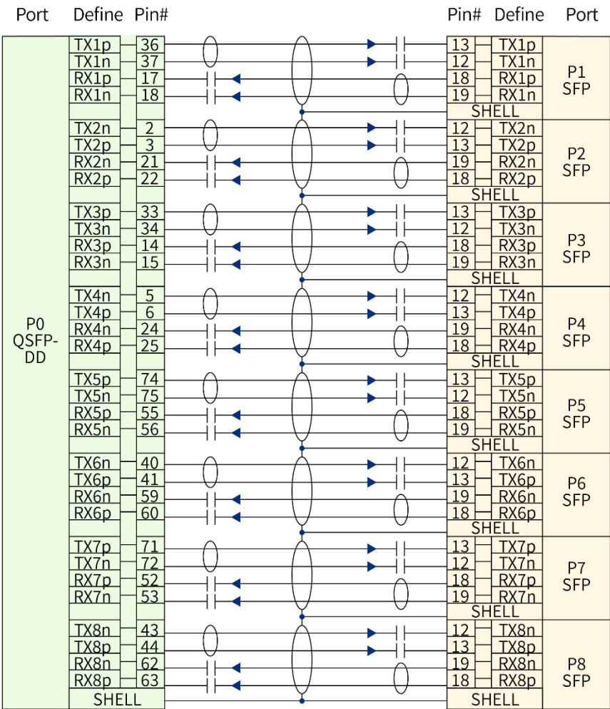
Figure 3 QSFP-DD 400G to 8*SFP56 Direct Attached cable Wiring
