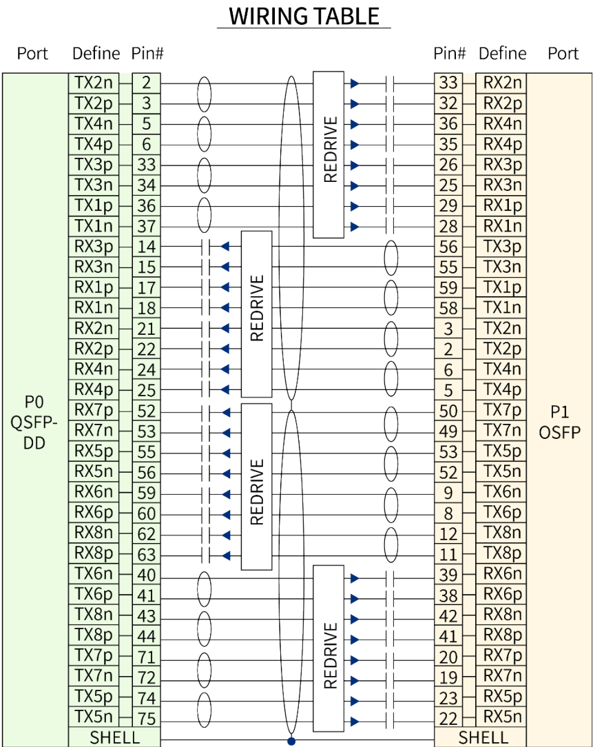
Figure 3 QSFP-DD 400G to OSFP/OSFP-RHS (400G) Active Redriver cable Wiring
