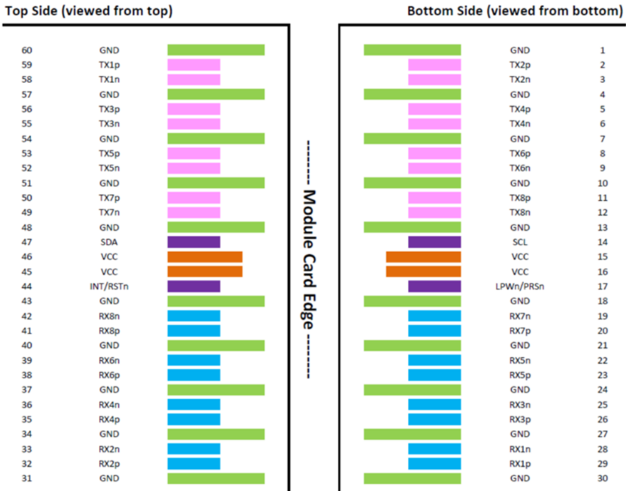
Figure 2 OSFP/OSFP RHS Module Contact Assignment
