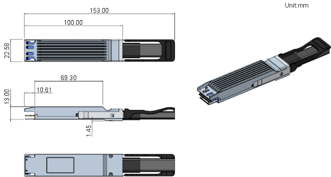
Figure 6 OSFP Form Factor
