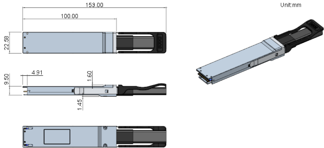
Figure 6 OSFP-RHS800 Form Factor (P1~P2 End)
