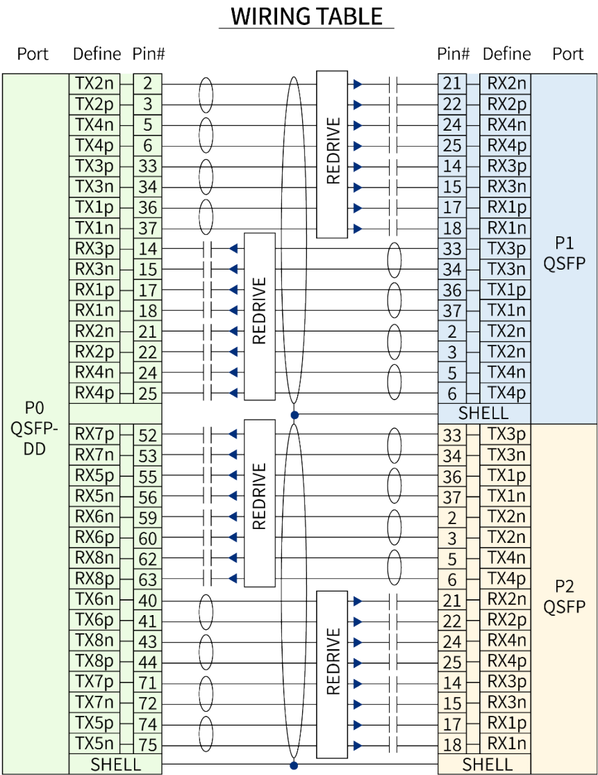
Figure 3 QSFP-DD 800G to 2*QSFP112 (4*100G) Active Redriver Cable Assembly Wiring
