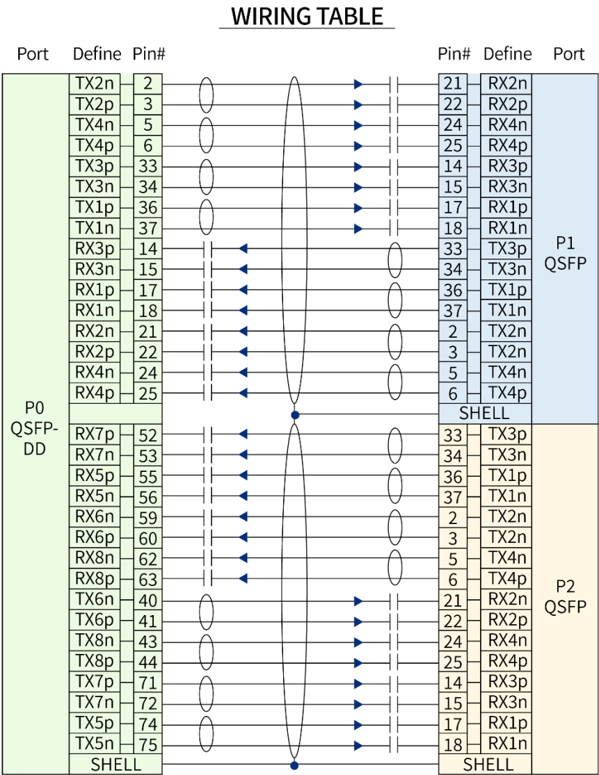
Figure 3 QSFP-DD 800G to 2*QSFP112 (4*100G) Direct Attached Cable Assembly Wiring
