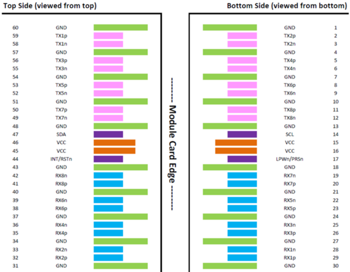
Figure 2 OSFP/OSFP RHS800 Module Contact Assignment
