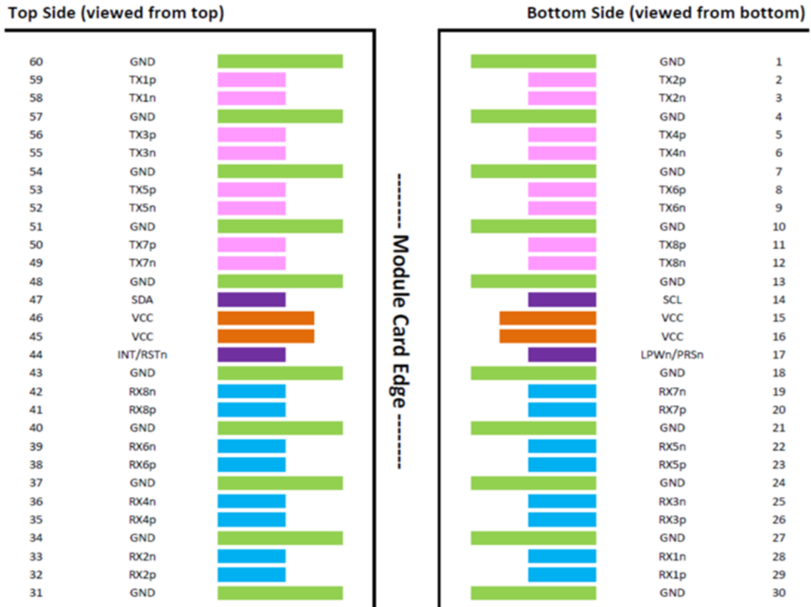
Figure 2 OSFP/OSFP RHS800 Module Contact Assignment
