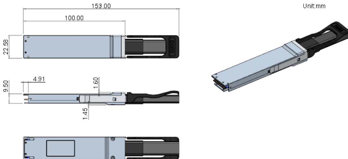
Figure 6 OSFP-RHS800 Form Factor (P1~P4 End)
