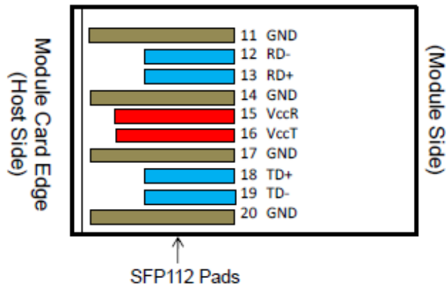
Figure 2 SFP112 Module Contact Assignment
