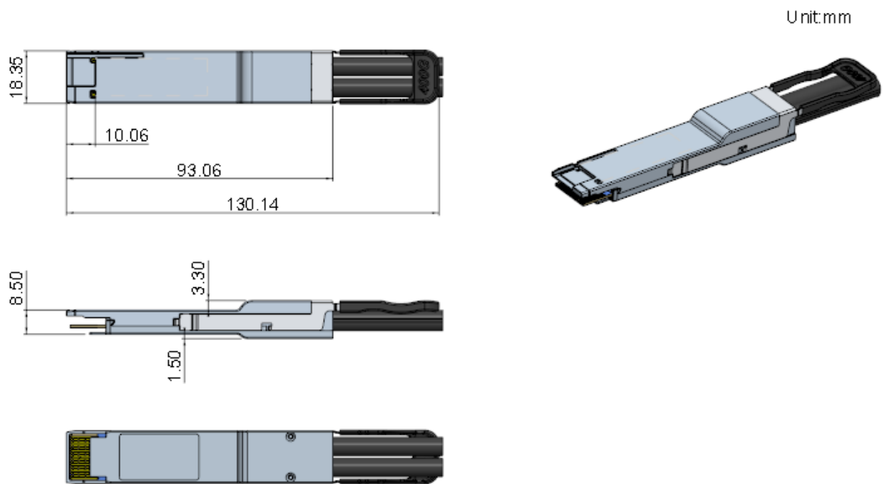
Figure 4 QSFP-DD 400 Form Factor
