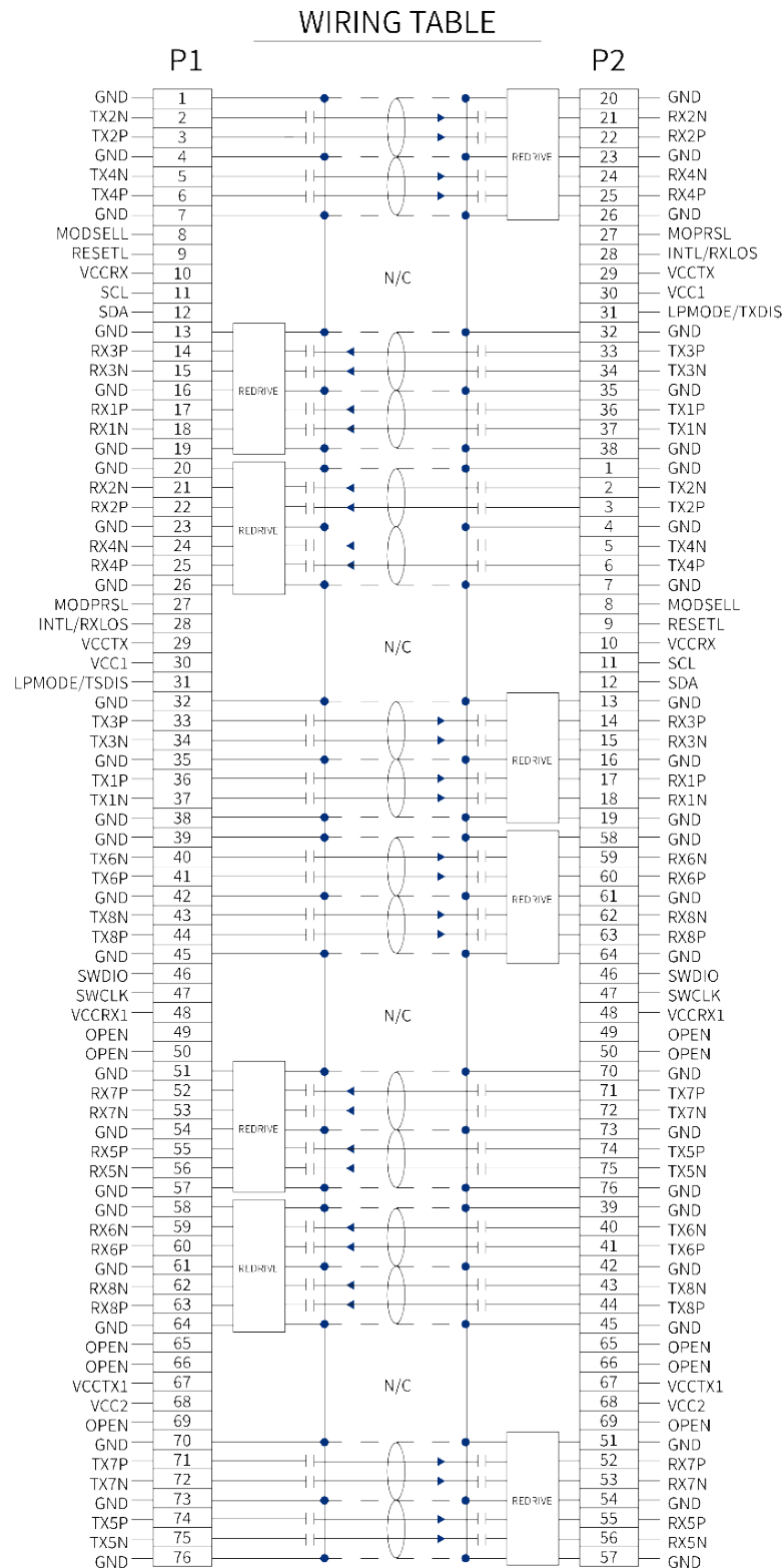
Figure 2 QSFP-DD800 to QSFP-DD800 800G Active Redriver Cable assembly Wiring
