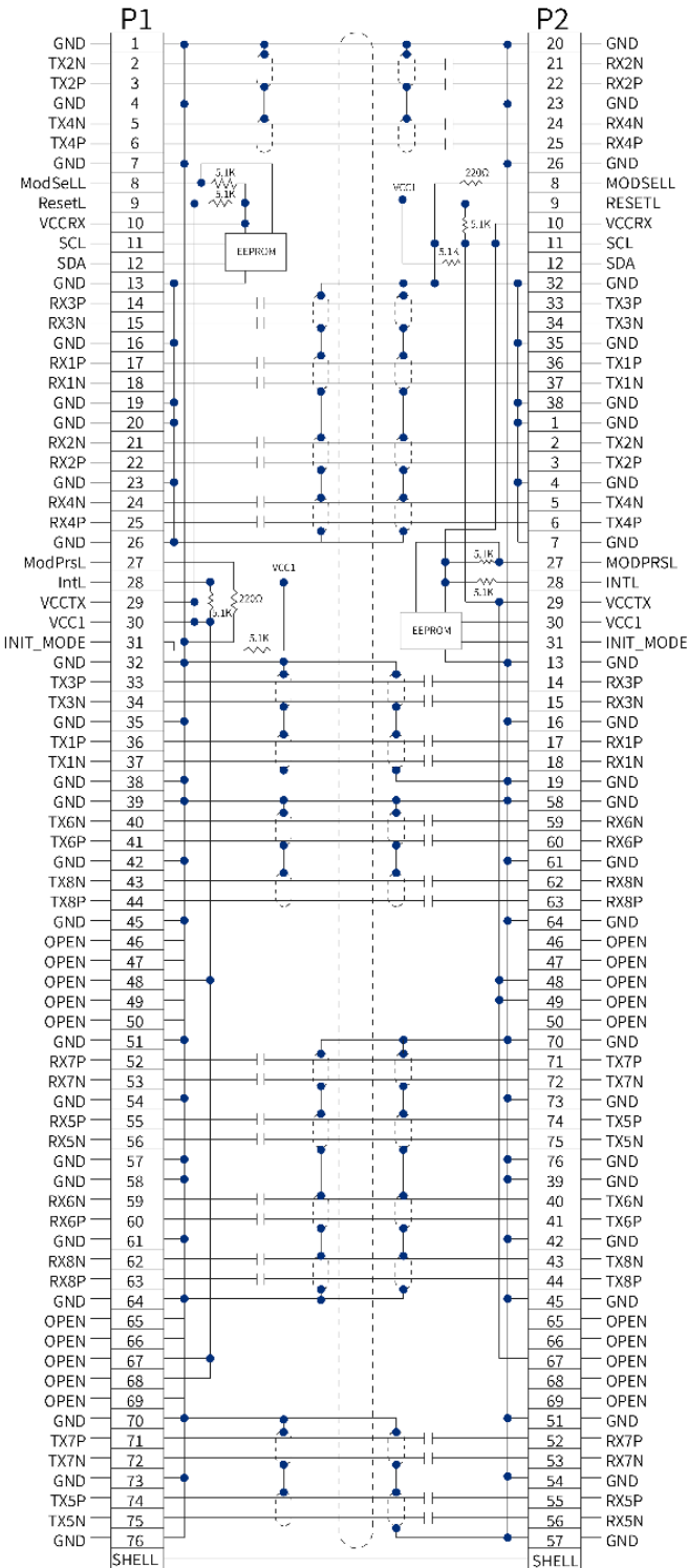
Figure 2 QSFP-DD800 to QSFP-DD800 800G Direct Attached Cable assembly Wiring
