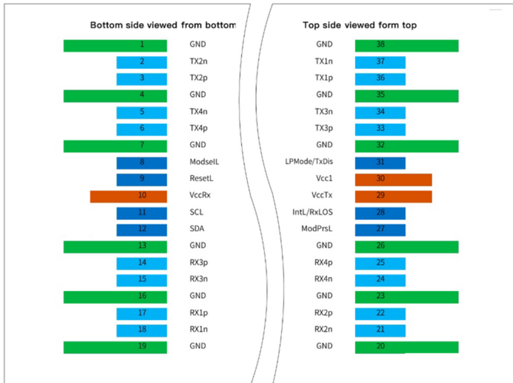
Figure 1 QSFP112 Module Contact Assignment
