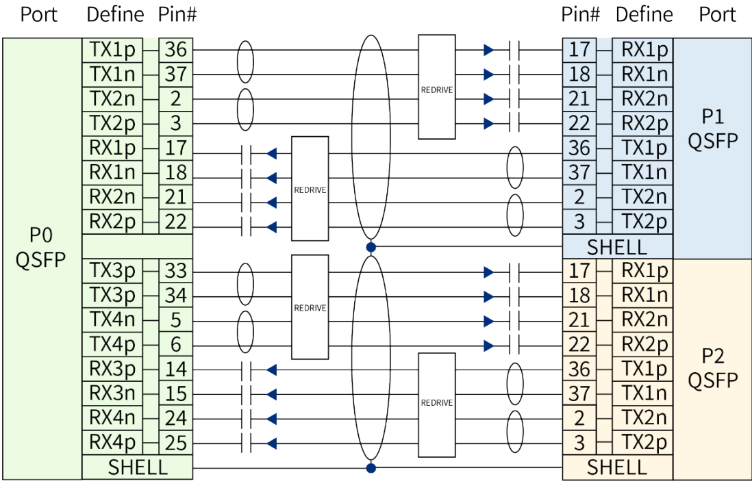
Figure 2 QSFP112 to 2*QSFP112 Active Cable assembly Wiring
