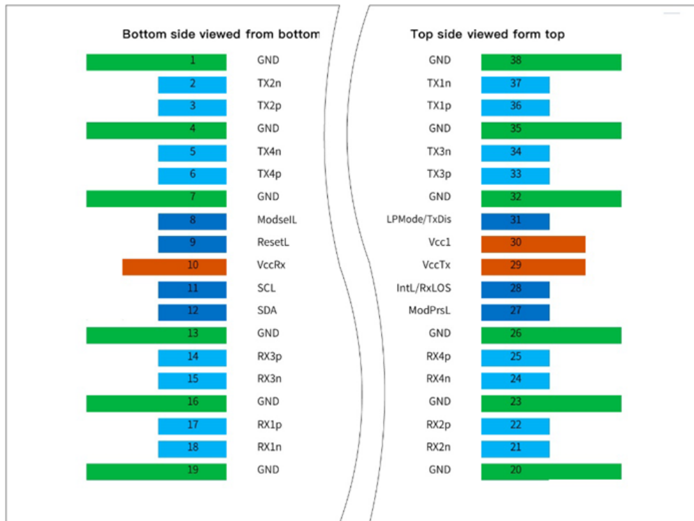
Figure 1 QSFP112 Module Contact Assignment
