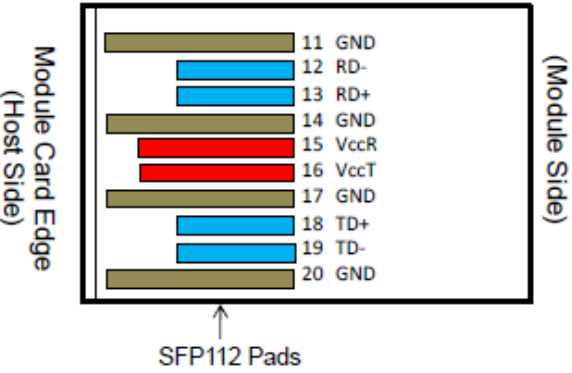
Figure 2 SFP112 Module Contact Assignment
