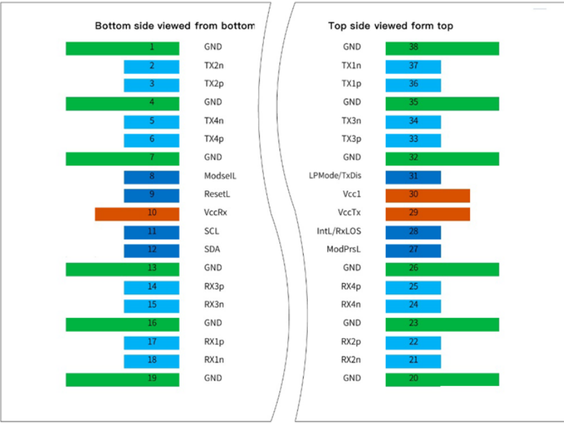
Figure 1 QSFP112 Module Contact Assignment
