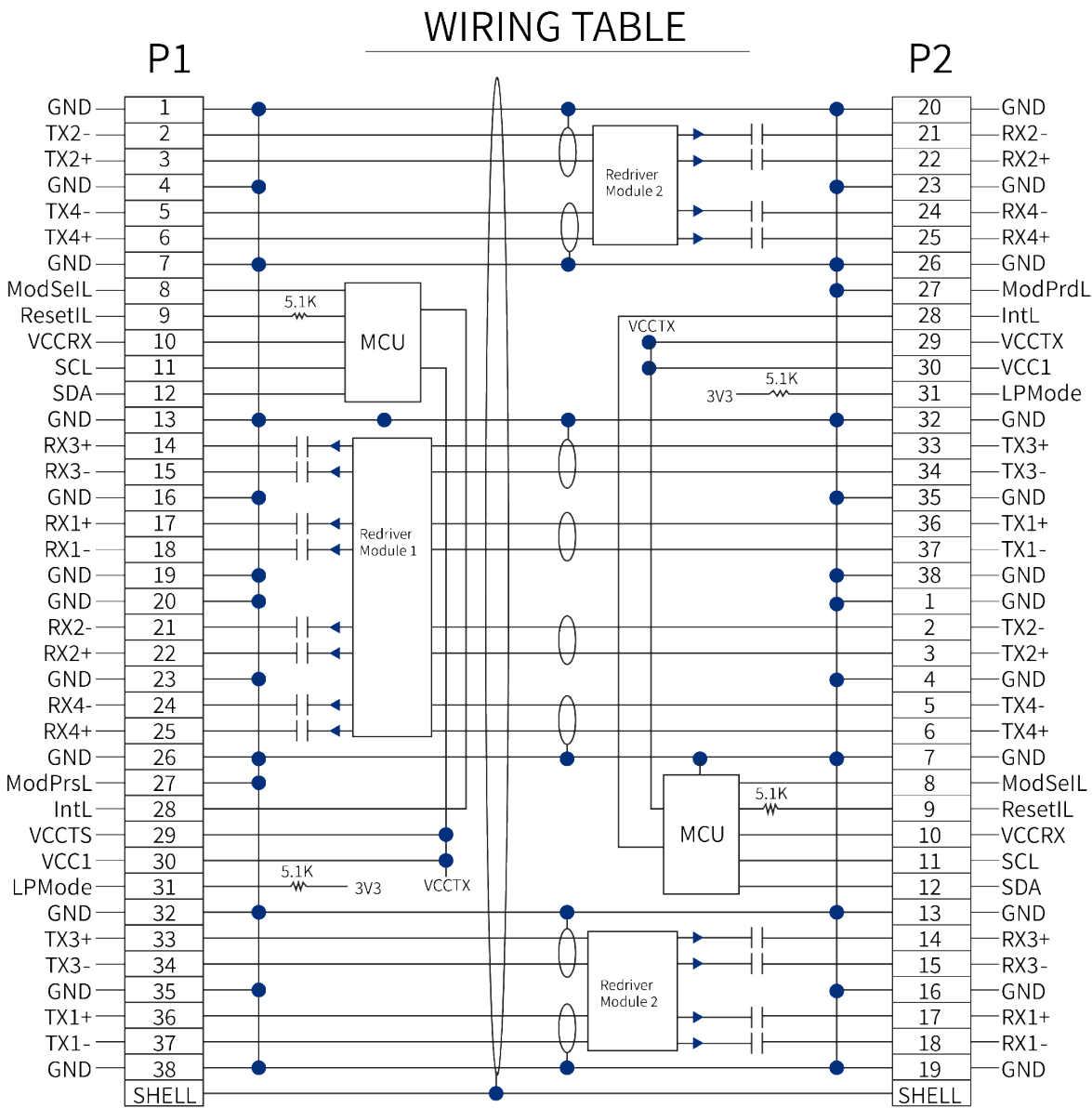
Figure 2 QSFP28(56) to QSFP28(56) Active Redriver Cable Assembly Wiring
