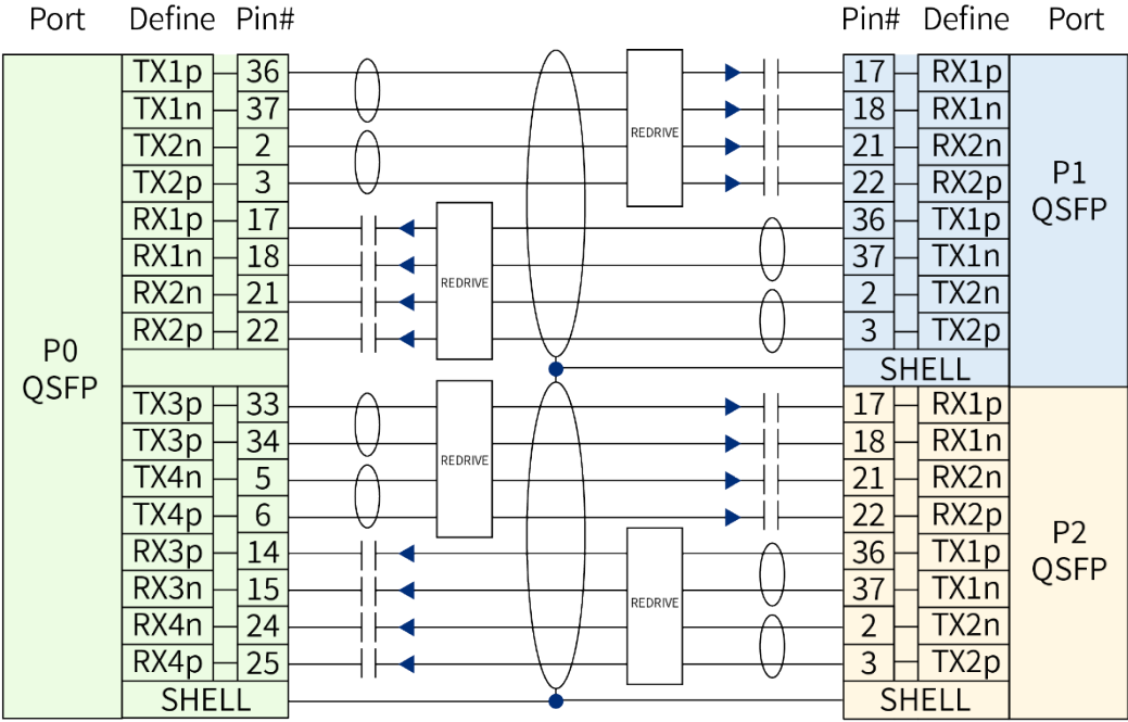
Figure 2 QSFP56(28) to 2*QSFP56(28) Active Redriver Cable Assembly Wiring
