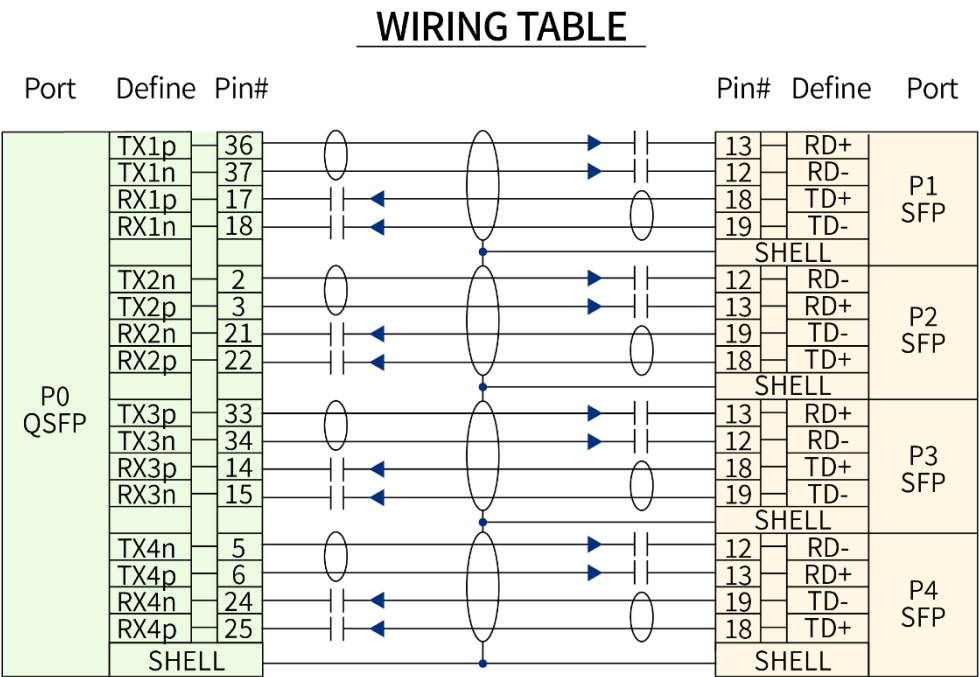
Figure 3 QSFP28(56) to 4*SFP28(56) Direct Attached Cable Assembly Wiring
