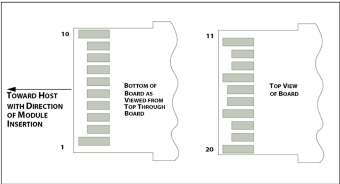
Figure 2 SFP28(56) Module Contact Assignment
